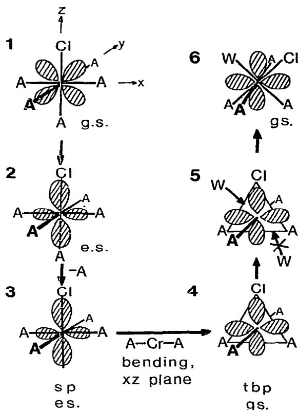
Fig. 1. Pictorial representation of the photostereochemistry of a Cr(III) complex according to the Vanquickenborne/Ceuleman's theory. (1) The ground state ( ^4B_1 ) of [\text{Cr}(\text{NH}_3)_5\text{Cl}]^{2+} (A = \text{NH}_3 ) with its occupied d_{xz} orbital shown. (2) Excitation to the lowest ^4E excited state corresponds to promotion of a d_{xz} or d_{yz} electron to a sigma antibonding orbital of mixed d_{z^2} and d_{x^2-y^2} character, ( d_{z^2-x^2} or d_{z^2-y^2} respectively, for the situation where all six ligands are equivalent). The figure shows the situation for that ^4E component corresponding to vacation of d_{xz} and occupancy of a ( d_{z^2-x^2} )-like orbital with >75\% d_{z^2} character (due to the smaller overall ligand sigma donor strength on the z axis in [\text{Cr}(\text{NH}_3)_5\text{Cl}]^{2+} { \epsilon_o(\text{NH}_3)=0.718 \mu\text{m}^{-1} , \epsilon_o(\text{Cl})=0.558 \mu\text{m}^{-1} }). This excitation labilizes the axial ( z axis) Cl and \text{NH}_3 ligands and to a lesser extent the x axis \text{NH}_3 ligands. (3) The preferential loss of the z axis ammonia ligand leads to a square pyramidal (sp) five coordinate intermediate (chloride apical) in its electronically excited state. This intermediate can lower its energy significantly by an allowed x axis \text{NH}_3\text{-Cr-NH}_3 bending downwards in the xz plane to yield (4). (4) The electronic ground state of a trigonal bipyramidal intermediate (tbp) with the chloride ligand in the equatorial plane. (5) Entry of a solvent molecule (W) in the equatorial plane of this ground state tbp intermediate trans to the chloride ligand is forbidden since it correlates with the excited state of trans - [\text{Cr}(\text{NH}_3)_4(\text{H}_2\text{O})\text{Cl}]^{2+} . In contrast, W entry cis to the equatorial chloride is allowed, as shown, as it correlates with (6), the ground state of the product cis - [\text{Cr}(\text{NH}_3)_4(\text{H}_2\text{O})\text{Cl}]^{2+} . Note that the excited state of this tbp intermediate has the d_{xz} orbital occupied and should show the opposite selection rule, therefore leading in theory to trans - [\text{Cr}(\text{NH}_3)_4(\text{H}_2\text{O})\text{Cl}]^{2+} product.
